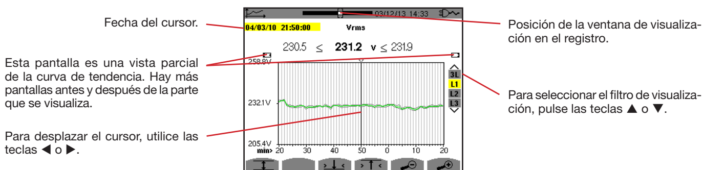
Figura 83: Vrms (L1) sin MIN-AVG-MAX
